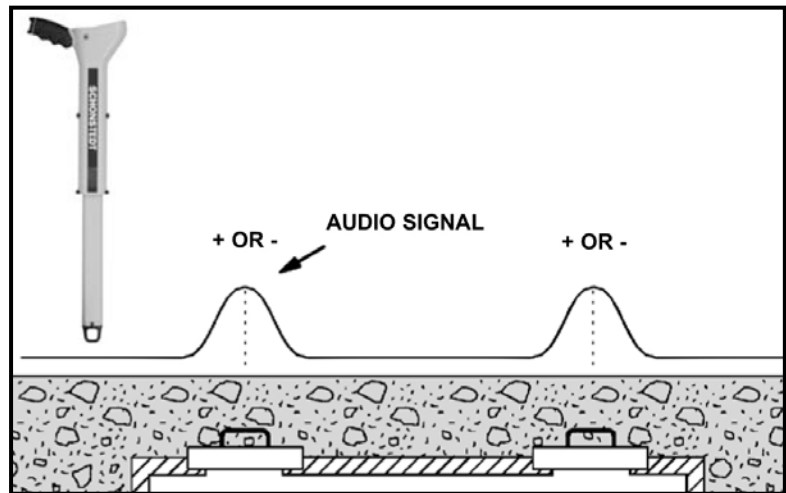
Figure 18. Signal Patterns Provided by Septic Tank Covers
