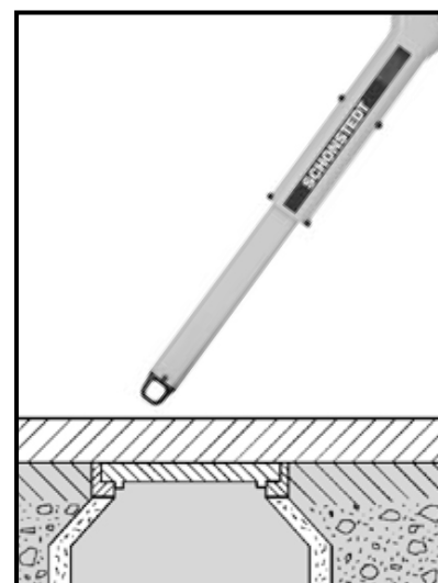
Figure 16. Locating Manhole Covers
