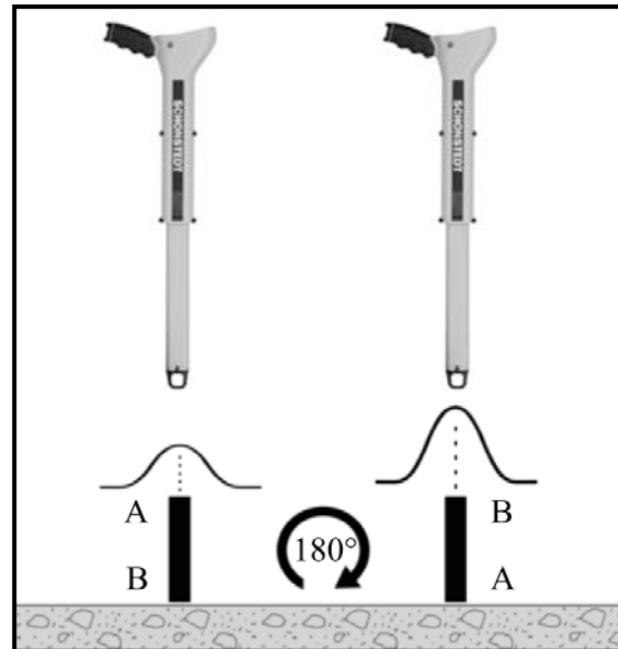
Figure 15. Checking a Stake's Orientation
