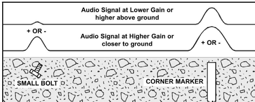
Figure 13. Decreasing gain Eliminates Unwanted Signals
