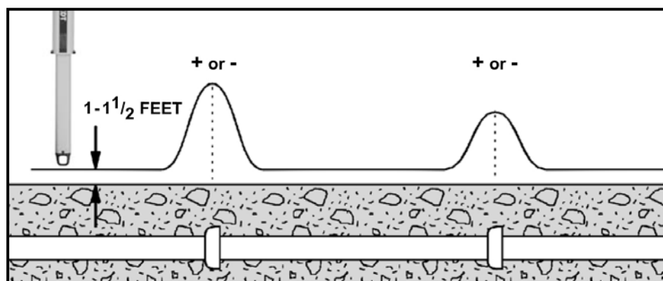
Figure 24. Signal Patterns Provided by Cast-Iron Pipes
