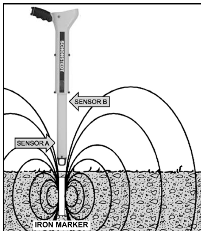
Figure 1. Detecting Magnetic Field of an Iron Marker
