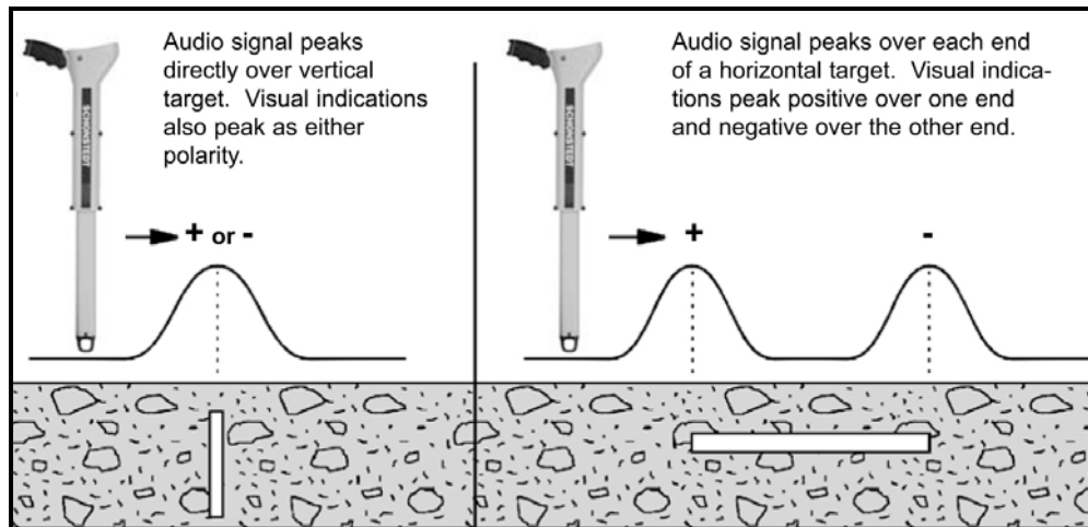
Figure 11. Signals from Vertical and Horizontal Targets
